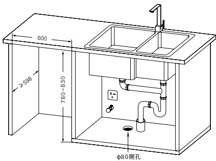
Φ80開孔
