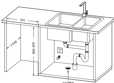
Φ80開孔
