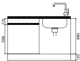
註：門片W596XH556mm
